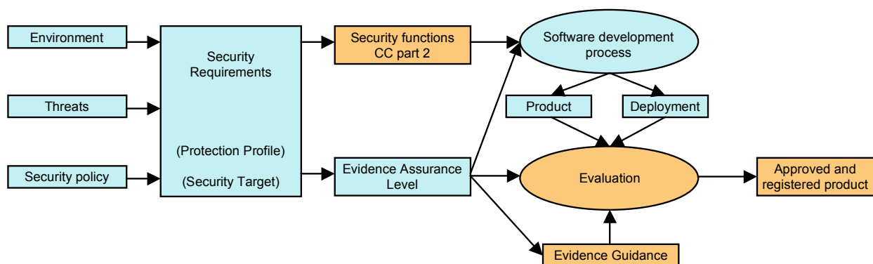
Figure 1: Overview Common Criteria.
